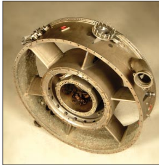
POWER PLANT MODULE
