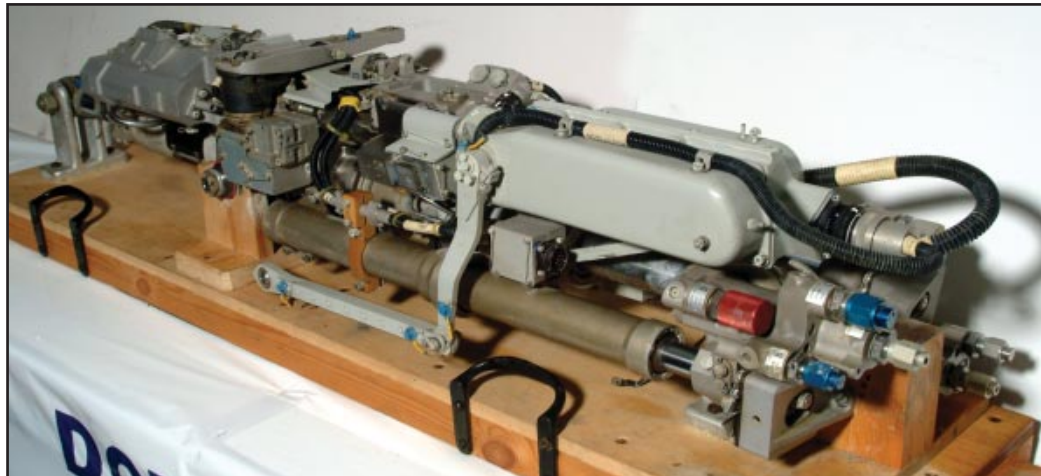
RUDDER POWERED FLYING CONTROL UNIT
